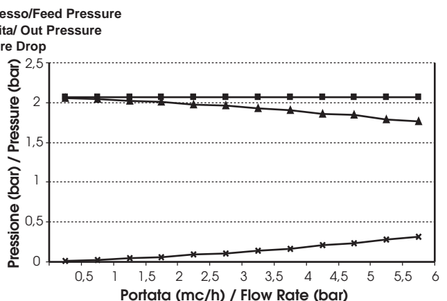
Cartuccia 9 3/4" FA-BIG 20 µ con filtro Aqua Big attacchi 1" / 9 3/4" FA-BIG 20 µ cartridge with 1" Aqua Big filter
